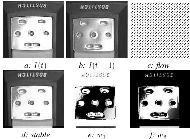
Figure 7: Specularity Experiment (a moving stapler).
