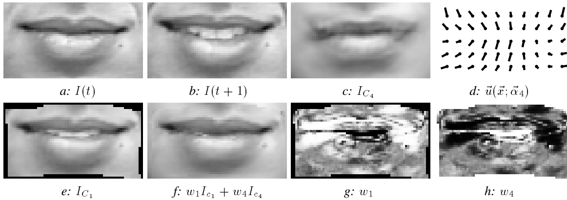
Figure 11: Facial Expression Experiment.
