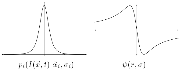
Figure 5: A robust likelihood p_i and \psi (the derivative of the log likelihood).
