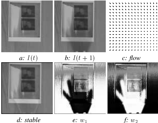
Figure 6: Illumination Experiment (cast shadow of a hand).
