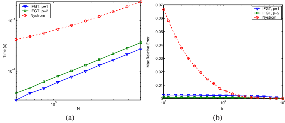
Figure 2: Performance comparison between the approximation methods. (a) Running time against N and (b) maximum relative error against k for fixed N = 1000 in 100 dimensions.
