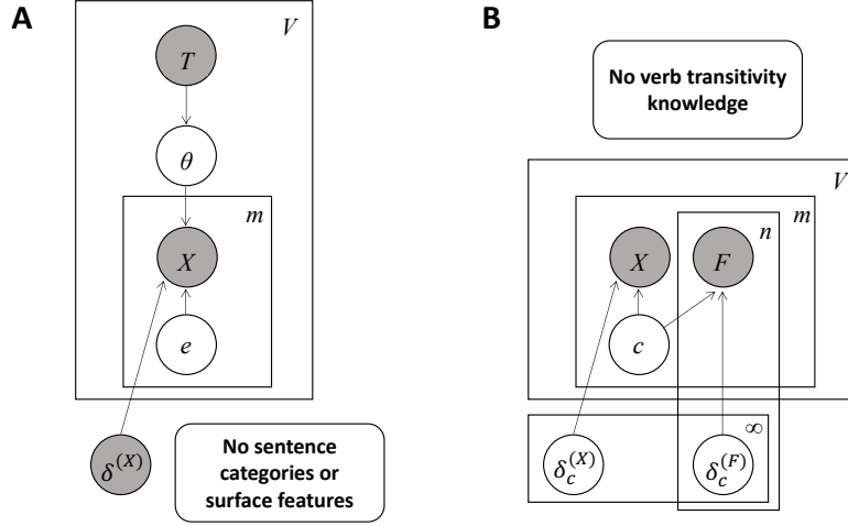
Figure 5. Graphical Models for (A) No-Category Baseline and (B) No-Transitivity Baseline
