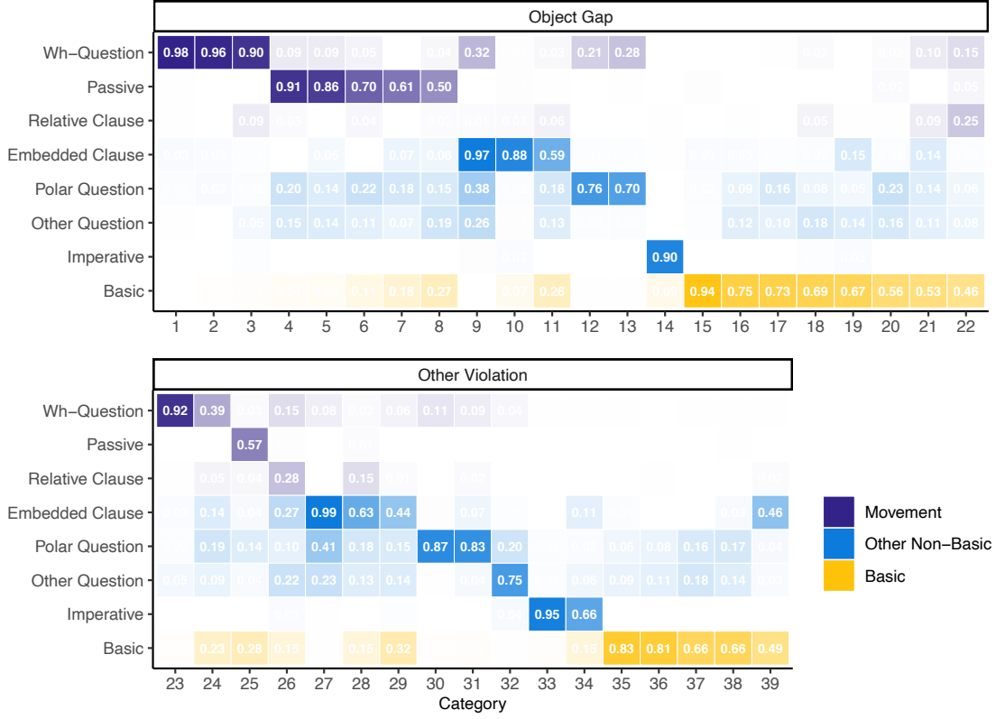
Figure 6. Proportions of Clause Types in Sentence Categories, No-Transitivity Baseline
