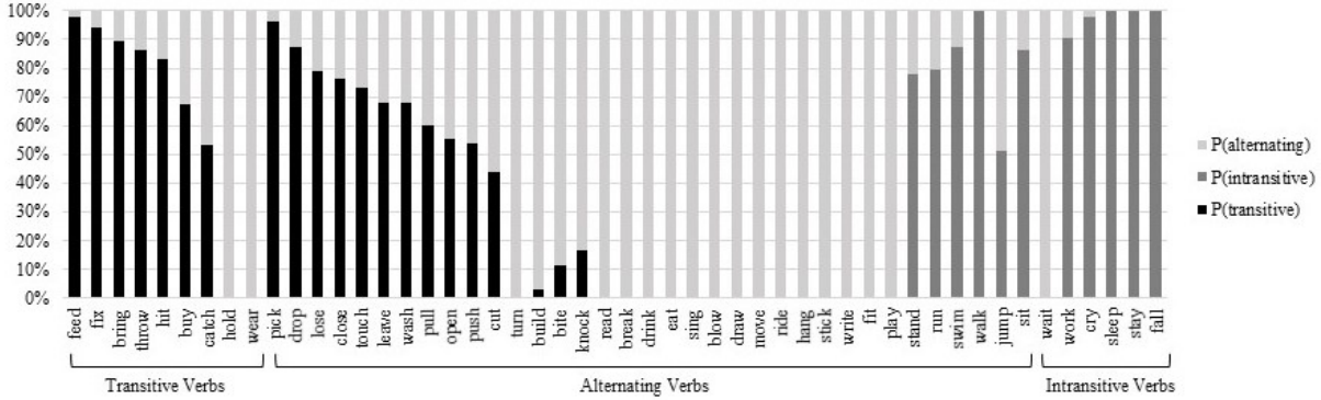
Figure 4: Posterior Distributions over Verb Categories ( T ), Oracle Model
