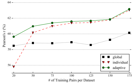
(a) Correlation.
