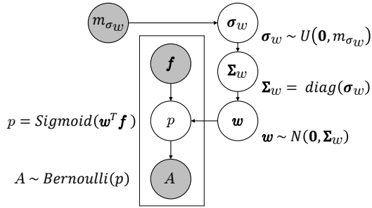
(b) Bayesian logistic regression for ASR.
