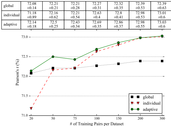
Figure 5: Results of adaptation to STS domains across different amounts of training data. Table shows mean \pm SD from 20 random train/test splits. While the baselines falter at extremes, the adaptive model shows consistent performance.
