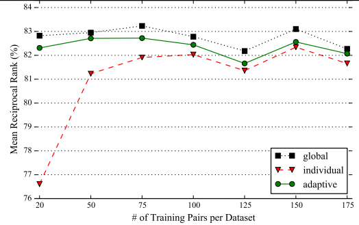
(b) Mean Reciprocal Rank.
