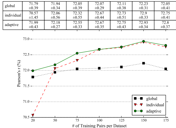
Figure 6: Multitask learning for STS: mean \pm SD from twenty random train/test splits. The adaptive model consistently performs well while the baselines have different failure modes.
