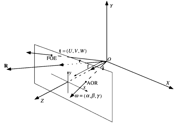
Figure 3. Image formation using perspective projection on a planar retina.
