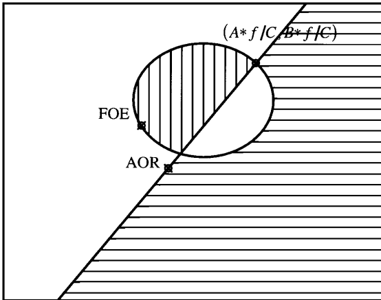
Figure 21. Separation of (A, B, C) coaxis vectors whose directions are shown in Fig. 20: A line passing through the AOR separates the positive and negative rotational components. A conic through the FOE separates the positive and negative translational components. In the area marked by horizontal lines all (A, B, C) coaxis vectors are greater than zero. In the area marked by vertical lines all (A, B, C) coaxis vectors are smaller than zero. The two other areas contain all the (A, B, C) coaxis vectors of length zero.
