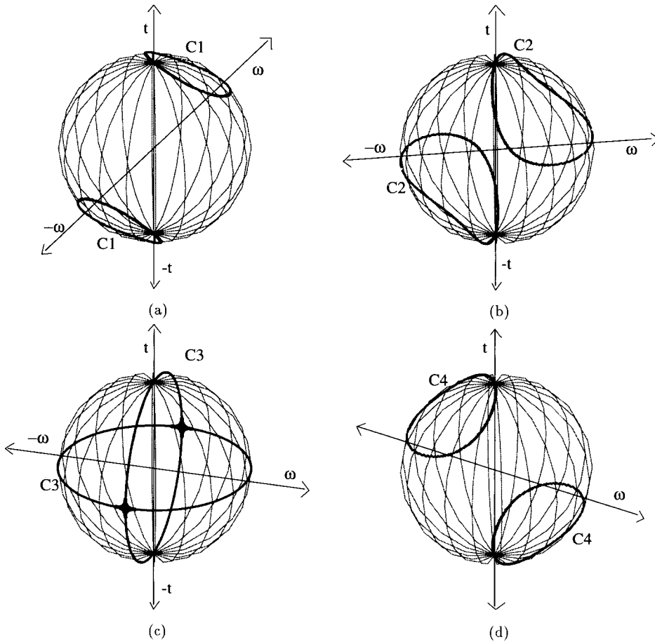
Figure 31. The locus of points on the sphere for which the motion vector could have the value (\mathbf{u} \cdot \mathbf{r})\mathbf{r} - \mathbf{u} constitutes second order curve(s). For the case of \mathbf{u} = 0 the locus is two curves which pass through the FOE and the AOR (and FOC and -AOR ). The four zero motion contours C_1 to C_4 displayed are defined by the same direction of translation ( \mathbf{t} ) and different directions of rotation ( \omega ), with the angle \alpha = \angle \mathbf{t}\omega increasing in value from C_1 to C_4 . In (a) and (b) for C_1 and C_2 we have \alpha < 90^\circ , in (c) for C_3 \alpha = 90^\circ , and in (d) for C_4 \alpha > 90^\circ .
