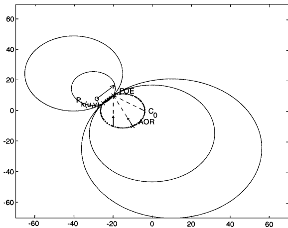
Figure 6. The motion vector in \mathbf{P}_{k(u,v)} is parallel to (u, v) . For every point on the zero motion contour the motion vector lies on a line connecting the point with the FOE.
