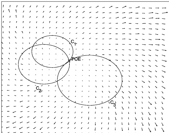
Figure 1. The rigid motion constrains the motion vectors to lie on conic sections in the image plane. C_1 , C_2 and C_3 are curves containing the motion vectors of values (0.5, 0.5) , (0.1, 0.7) , and (-0.4, -0.4) .
