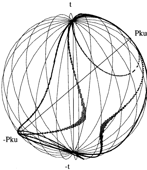
Figure 34. For the general case all k\mathbf{u} iso-motion contours intersect in four points; the FOE, the FOC, and the points \mathbf{P}_{k\mathbf{u}} and -\mathbf{P}_{k\mathbf{u}} .
