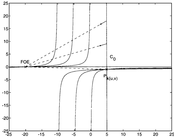
Figure 10. Iso-motion contours for fixating stereo: For all points along a line parallel to the Y -axis the motion vectors are in the direction of their translational motion components.
