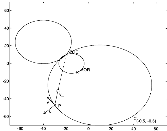
Figure 7. For any point \mathbf{P} with motion vector \mathbf{v} on a general \mathbf{u} iso-motion contour the motion vectors \mathbf{v}_- , where \mathbf{v}_- = \mathbf{v} - \mathbf{u} , is parallel to the translational component \mathbf{v} .
