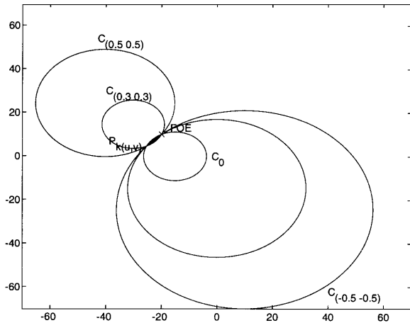
Figure 5. The family \phi(x, y, u, v, k) of iso-motion contours intersect at two points on the zero motion contour: The FOE and \mathbf{P}_{k(u,v)} .
