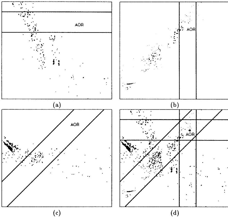
Figure 29. Localization of the AOR from normal flow vectors of (A, B, 0) coaxis vectors of length zero through the location of areas where bands are thinnest, (a) (1, 0, 0) coaxis vectors (red), (b) (0, 1, 0) coaxis vectors (green), (c) (0.707, 0.707, 0) coaxis vectors (blue), (d) the intersection of the areas found in (a), (b), and (c) provides a bounded area for the location of the AOR.
