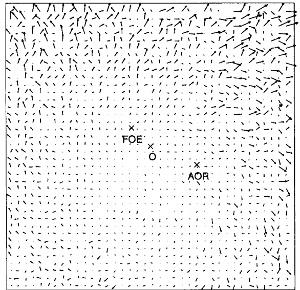
Figure 23. Synthetic normal motion field used as input data for the localization of the FOE and AOR shown in the next three figures.
