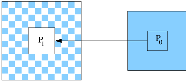
Figure 5: Simple example of the Growing Squares technique with two processes.
