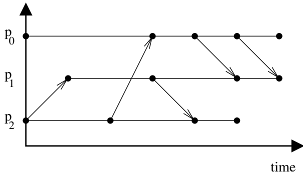
Figure 1: Hasse diagram visualization with 3 processes.
