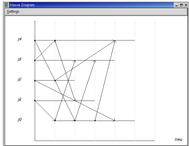
Figure 4: CausalViz Hasse visualization.
