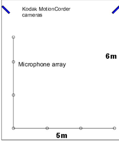
Figure 1: Schematic of flight room experimental set up.
