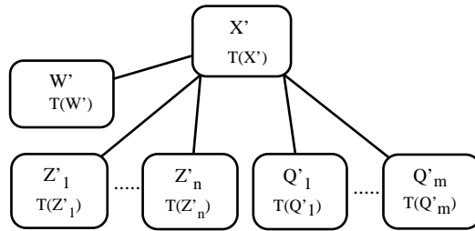
Figure 2 Formal Definition of Lexical Conceptual Structure
