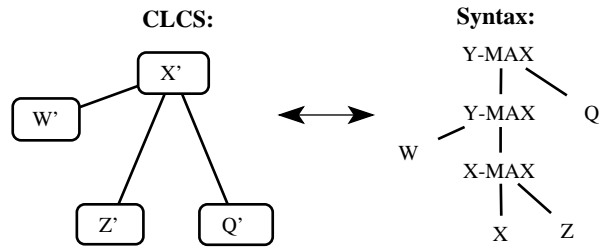
Figure 8 GLR Mapping between the CLCS and the Syntactic Structure
