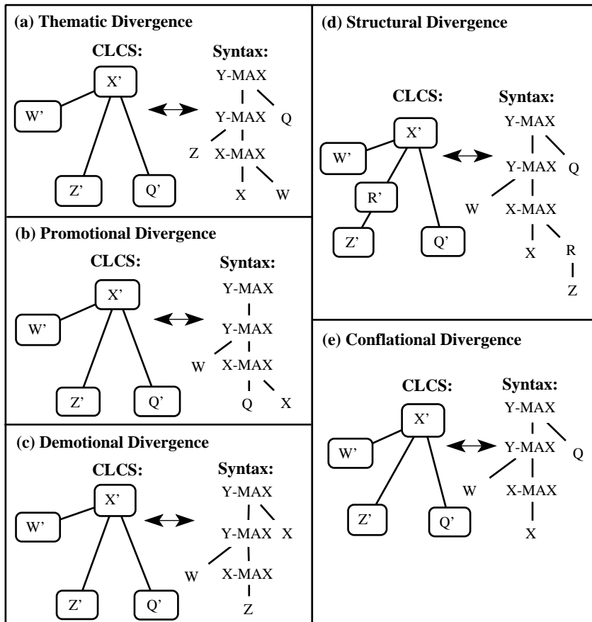
Figure 9 Translation Mappings for Cases where GLR Default Positions are Overridden
