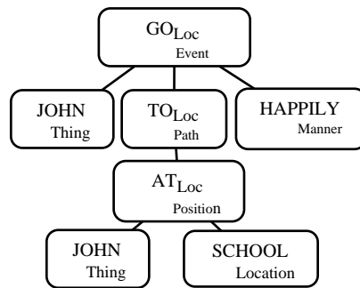
Figure 3 CLCS Representation for John went happily to school
