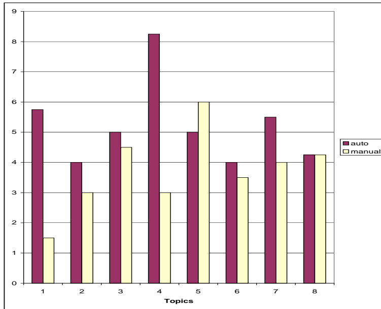
Fig. 4. Average number of query iterations, by topic.
