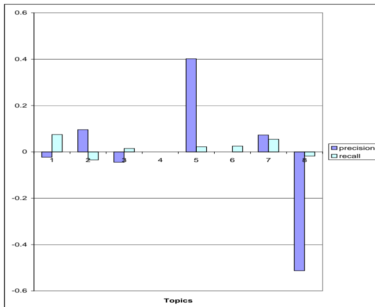
Fig. 3. Absolute improvement in precision and recall from the manual condition, strict judgement. Bars above the x axis favor the manual condition, below favor the automatic condition.
