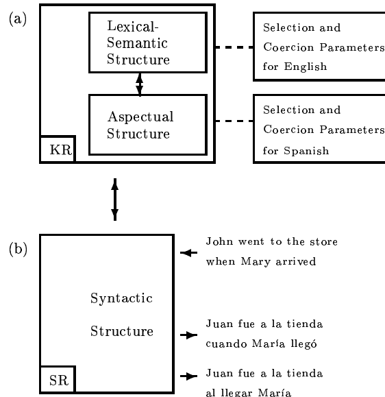
Figure 2: Overall Design of UNITRAN
