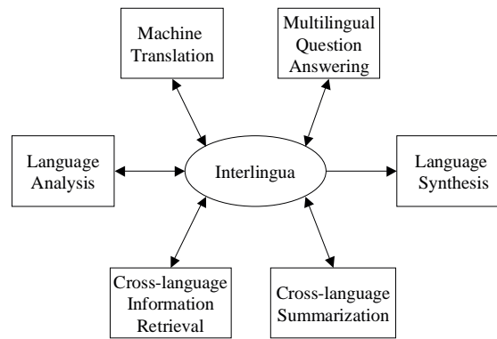
Figure 2: Use of Interlingua in Multiple Applications
